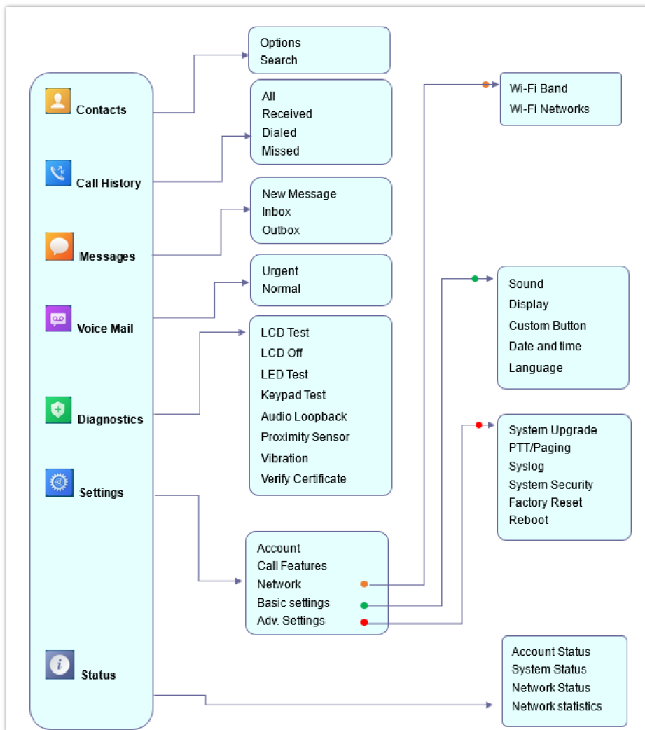
Figure 9: Menu Structure
